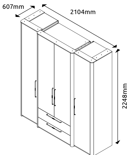
P42/AI LWH - 2104x607x2248
