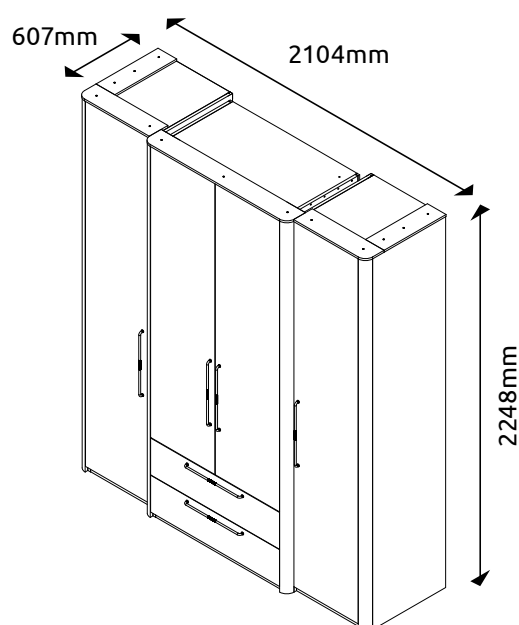
P42-2OG/AI LWH - 2104x607x2248
