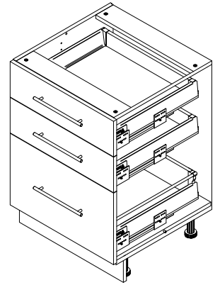
R-60-3MBOX LWH - 600X840X600
