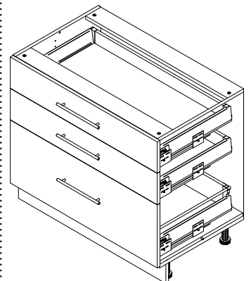
R-90-3MBOX LWH - 900x840x600
