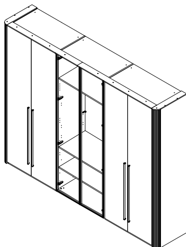
P6-2AL/RO LWH - 2880X559X2248
