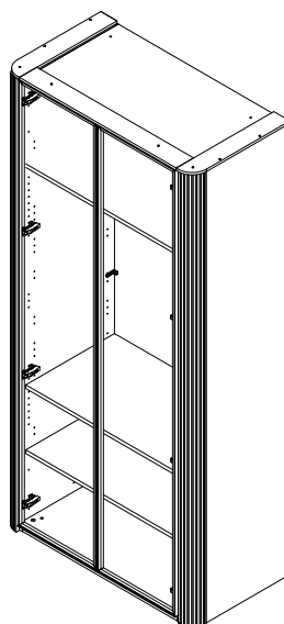
P2-2AL/RO LWH - 1080X559X2248
