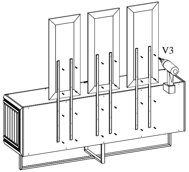
Practice for connection to the wall
