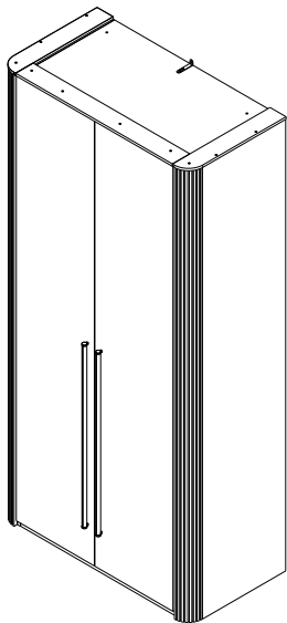
P2/RO LWH - 1080X559X2248
