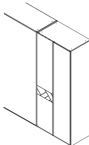
DP2-10G/AV LWH - 900x555x2236
