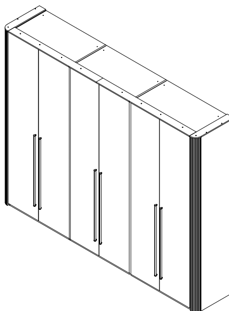
P6R/RO LWH - 1280X559X2248
