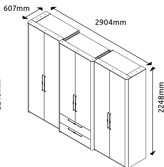
P62-2OG/AI LWH - 2904x607x2248
