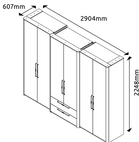
P62/AI LWH - 2904x607x2248
