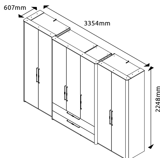
P72-3OG/AI LWH - 3354x607x2248
