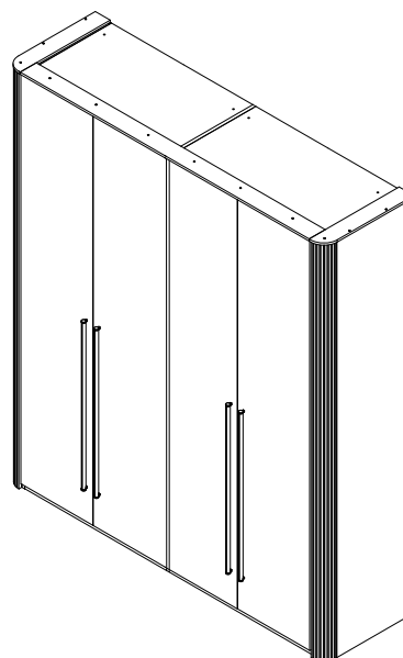
P4R/RO LWH - 1980X559X2248
