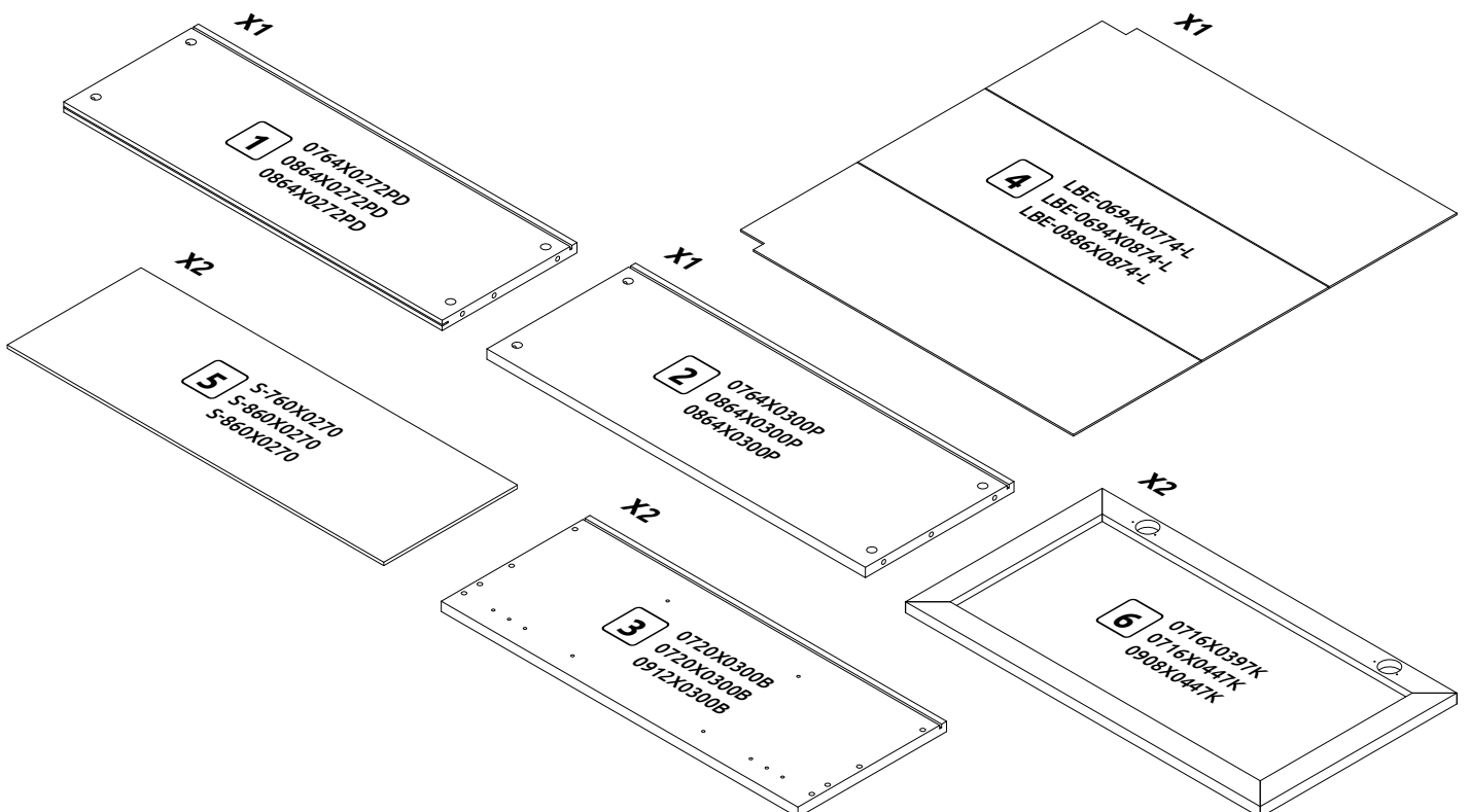
V7-80-2AL LHW-800x720x320
